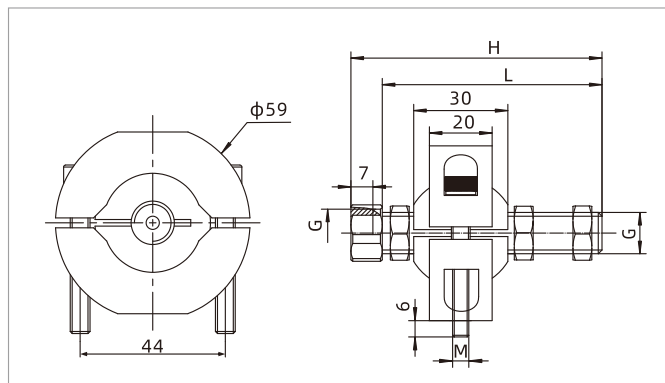
PJH-2□□
