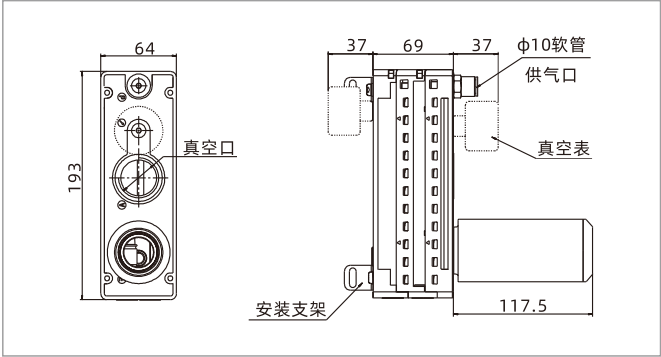
AMC75-100
