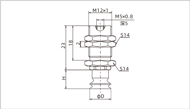
SP3B□□-M5F-M12M
